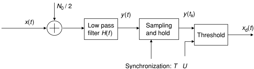
Figure A.4 A binary receiver
