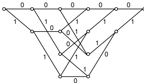
Figure 7.5 A trellis for the block code C_b(5, 3)
