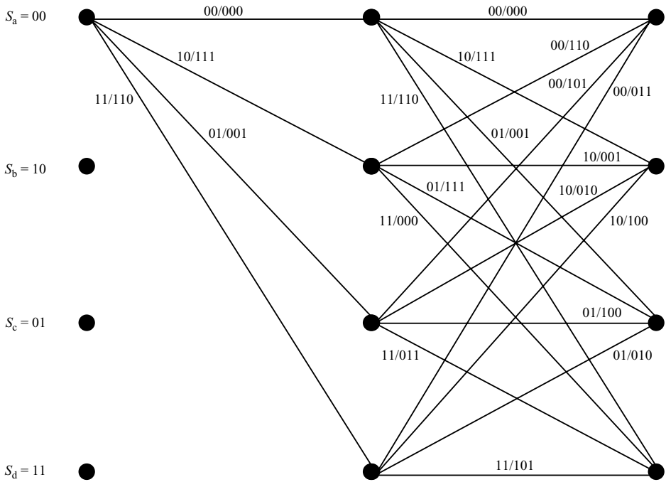
Figure 6.34 Trellis for a convolutional code of rate R_c = 2/3 constructed in the traditional way
