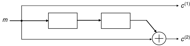
Figure 6.2 Structure of a systematic convolutional encoder of rate R_c = 1/2
