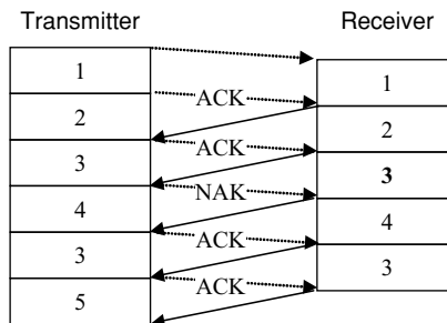
Figure 2.7 Selective-repeat ARQ scheme
