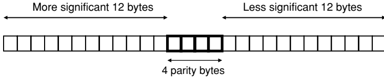
Figure 5.4 Code vector generated by the shortened RS code C_{RS}(28, 24)
