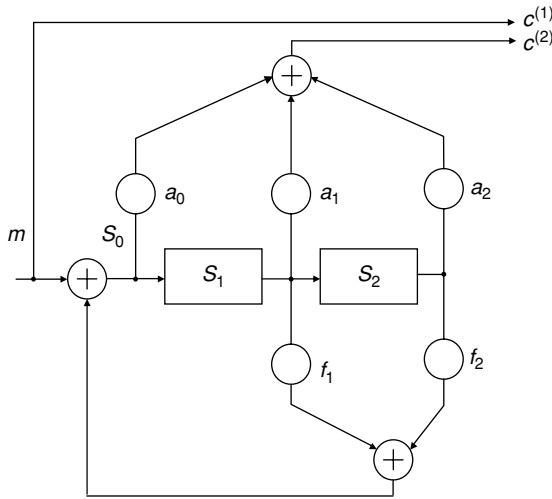
Figure P.6.6 Convolutional encoder, Problem 6.8
