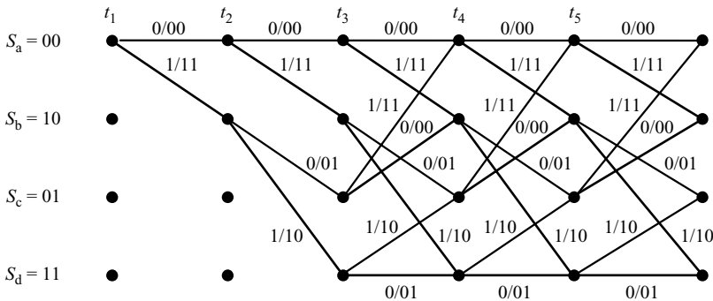
Figure 6.13 Trellis for the convolutional encoder of Figure 6.12
