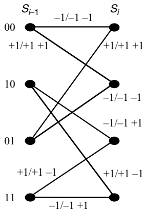
Figure 7.14 Trellis with transition information in polar format
